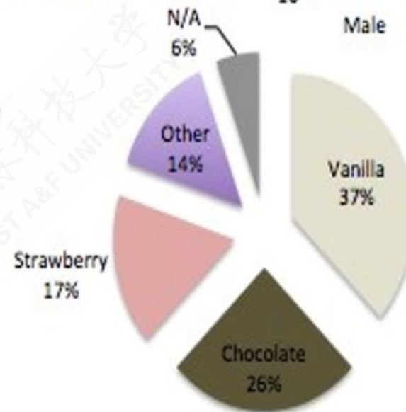
Descriptive Statistics
